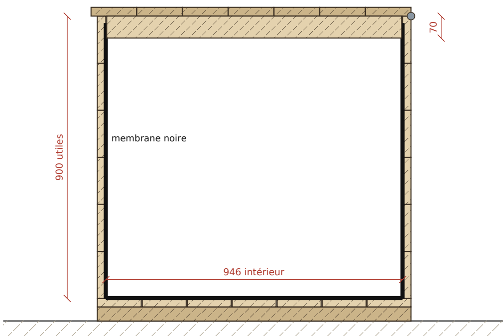
COUPE A-A (plan x = 0) 1:12
