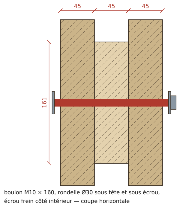
D1 — JOINT PIED / TRAVERSES 1:3
